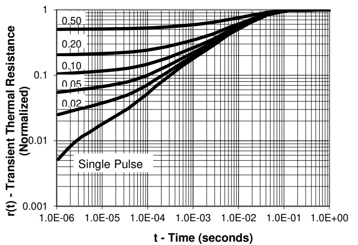
Transient Thermal Response, Junction-to-Ambient
